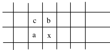
Figure 7.7 Spatial relation between the pixel to be coded and three decoded neighbors
