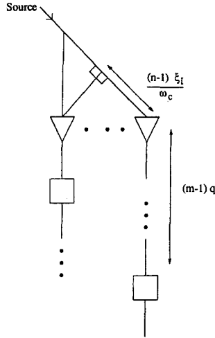
Fig. 1. Computation of time delay in STAP.
