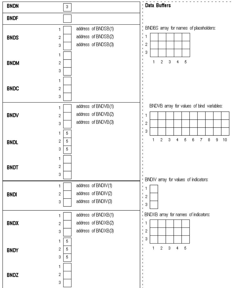
Figure 4-4 Initialized Bind Descriptor
