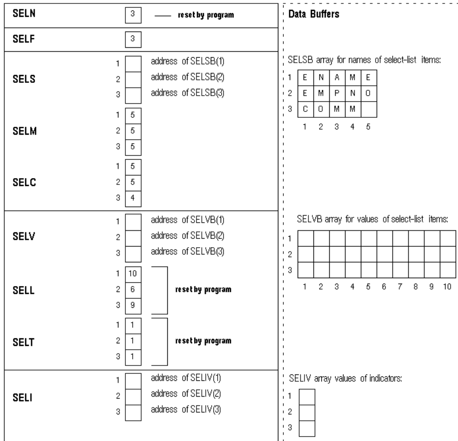
Figure 4–8 Select Descriptor before the FETCH
