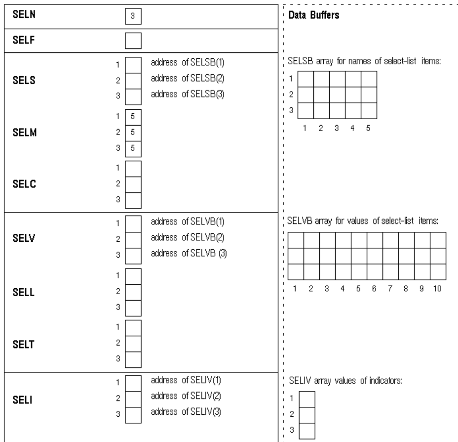
Figure 4-3 Initialized Select Descriptor
