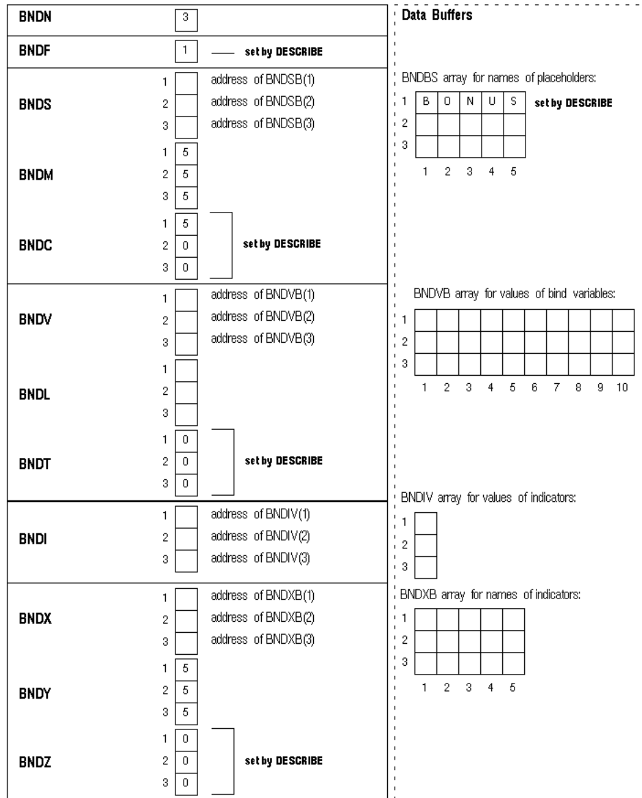
Figure 4-5 Bind Descriptor after the DESCRIBE
