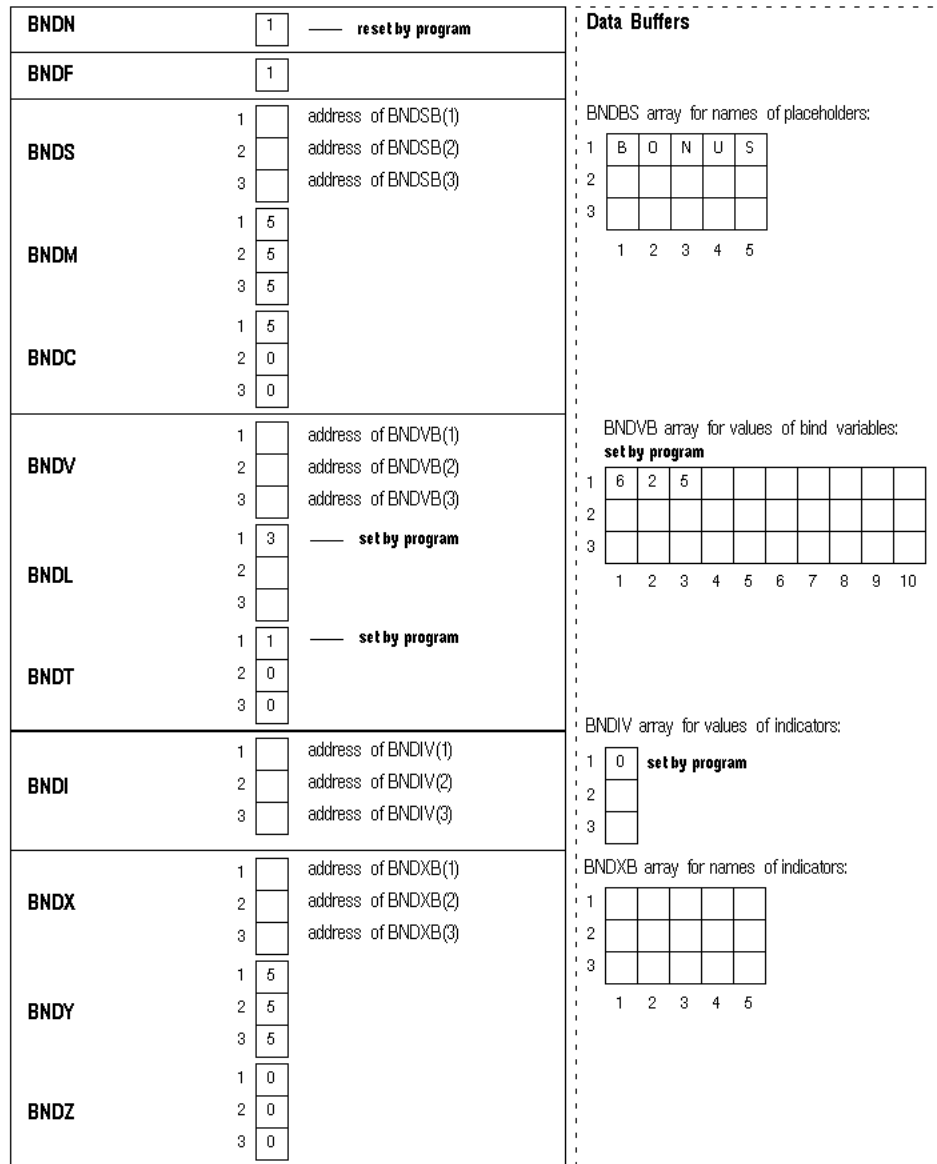
Figure 4-6 Bind Descriptor After Assigning Values
